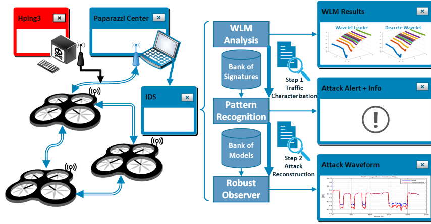
Fig. 1. General framework of the proposed IDS system
