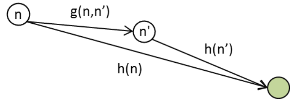
Fig. 2. Triangle Inequality Condition for Consistent Heuristics
