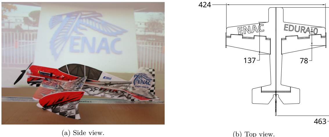
Figure 2: Side view (a) of the EDURA-0 vehicle based on an E-flite UMX Yak 54 3D commercial-off-the-shell aircraft; and CAD drawing (b) from the top with measures: wing span, root chord, tip chord, and length (Quantities in millimetres).
