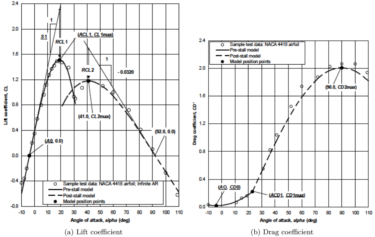
Figure 6: Fitting of lift and drag coefficients by the AERODAS model of Spera 2008, 23 Fig. 2.
