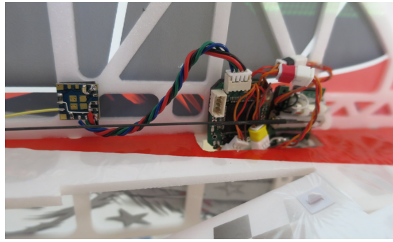
Figure 3: Autopilot configuration (from left to right): ESP8266-9 wifi module, Lisa-MXs board, and the linear servo for the elevator.
