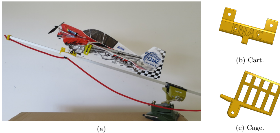
Figure 4: The EDURA catapult launcher with aircraft (a) and the main components in CAD.
