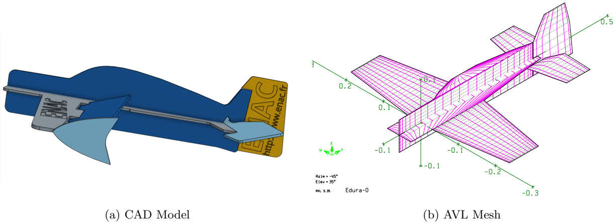
Figure 5: CAD model of the EDURA-0 aircraft and its control surfaces(a) and AVL Mesh(b).
