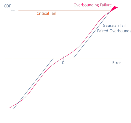
Figure 4: Overbounding Failure
