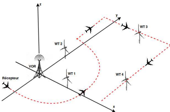
Fig. 2. Configuration.
