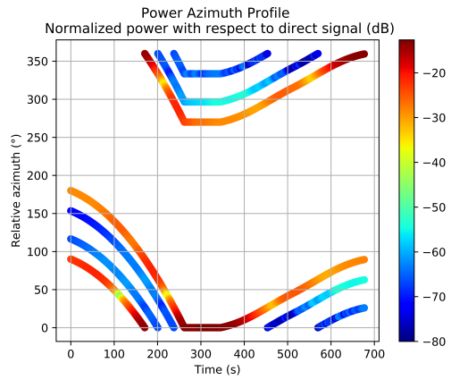
Fig. 4. Power Azimuth Profile of the multipath along the trajectory.
