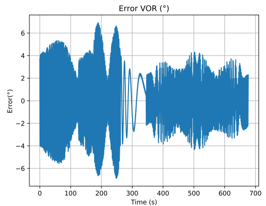
Fig. 5. VOR Error along the trajectory.
