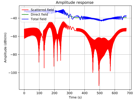
Fig. 3. Electric field (dBV/m) along the aircraft trajectory.
