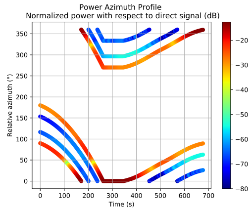
Fig. 4. Power Azimuth Profile of the multipath along the trajectory.
