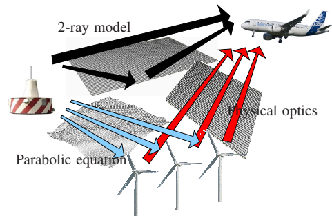
Fig. 1. Overview of the method to compute multipath.
