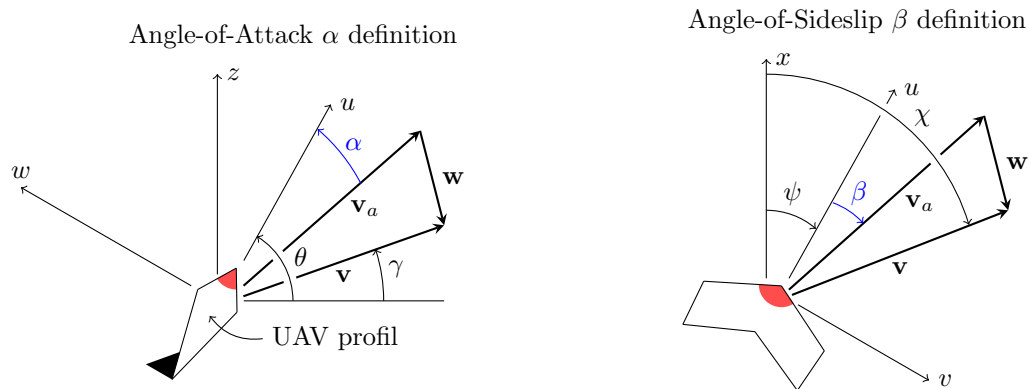
Figure 2. The wind triangle relationship between ground speed v , airspeed v_a and wind w , projected, respectively, onto the vertical (at left) and horizontal (at right) planes, making in evidence the Angle-of-Attack \alpha and the Angle-of-Sideslip \beta . The direction of the ground speed is specified using the course \chi , which represents the angle between the projection of v onto the xy -plane and north (i.e., the direction of travel relative to the Earth’s surface) and the flight path \gamma which is the angle between the xy -plane and v . The pitch \theta moves the UAV nose up or down and heading (yaw) \psi is the direction that the UAV is pointed. In the absence of wind, the difference between course and heading, the so-called crab-angle, is the Angle-of-Sideslip.
