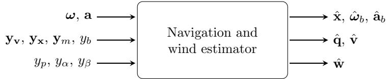
Figure 4. Tightly coupled approach. The only estimator obtains both navigation state and wind estimates, from all the available measurements, introducing thus correlation between estimated variables.
