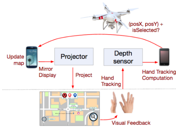
Figure 4. FlyMap Outdoor Architecture with the two hand gestures used for input.
