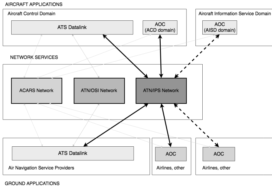
Fig. 2. ATN/IPS implementation (from [4])
