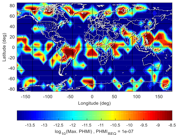
Figure 7 - Maximum PHMI in log scale based on the alert limit for RNP 0.3 operation (i.e., 556m).
