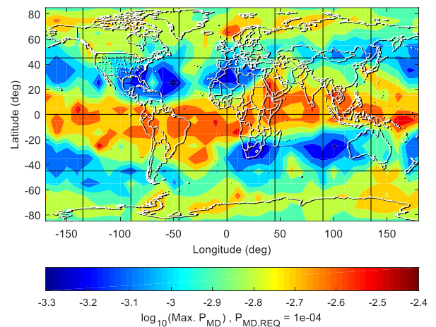
Figure 2 - Maximum PMD against dual failures obtained when the GPS/GLONASS MOPS test method is applied to PMD evaluation. The highest PMD is represented in log scale.
