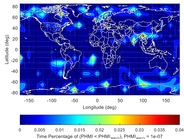
Figure 5 - Percentage of time that the evaluated PHMI is lower than the associated requirement of 10^{-7} .
