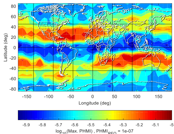
Figure 4 - Maximum PHMI under multiple failure modes when the horizontal user protection bound based on the proposed MOPS test procedure is applied. Each maximum value is expressed in log scale.
