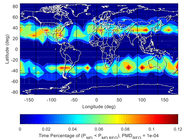
Figure 3 - Percentage of time that the evaluated PMD is lower than the associated probability of missed detection requirement of 10^{-4} .
