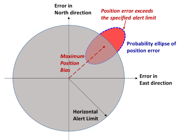
Figure 1 – Position error probability distribution and protection region
