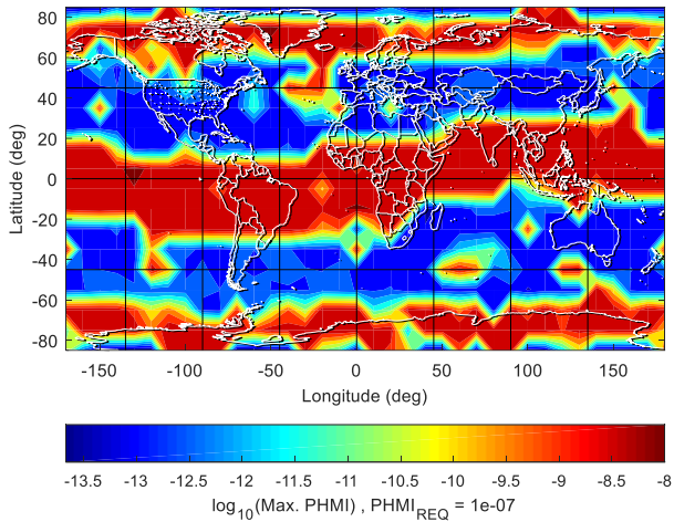
Figure 6 - Maximum PHMI in log scale obtained using the multi-bias RAIM protection bound with the measurement noise protection. The maximum goes up to approximately 2 \cdot 10^{-8} .
