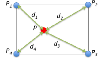
Fig. 1: Metric interpolation
