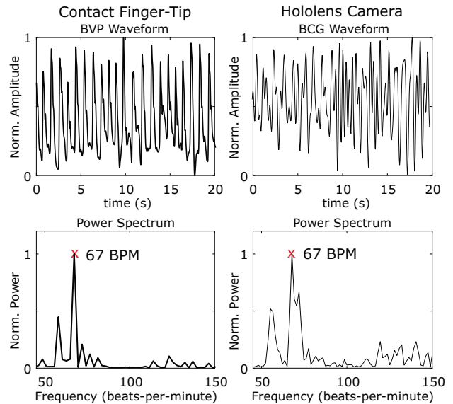
Figure 6: Examples of pulse waveforms from the finger-tip sensor and iBCG measurements. Top) The BCG waveform from the HoloLens and the PPG waveform from the finger-tip sensor. Bottom) The power spectra of the signals and the detected HR.
