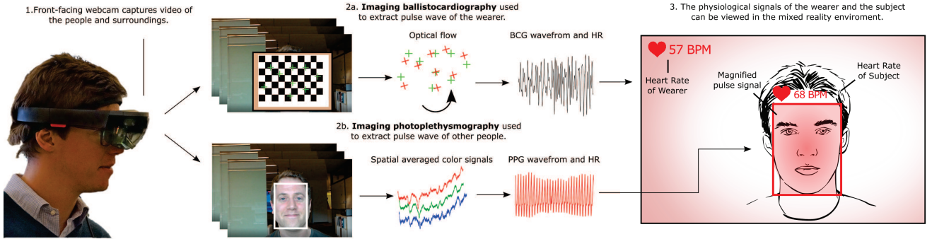
Figure 2: Schematic of the Cardiolens system. Images from the front-facing camera are used to extract the physiological state of the wearer and the person they are looking at. Imaging photoplethysmography is used to recover the pulse wave of the person being looked at. Imaging ballistocardiography is used to recover the pulse wave of the wearer. These signals are used to augment the appearance of the real-world allowing the wearer to see the normally “hidden” physiological information in real-time.
