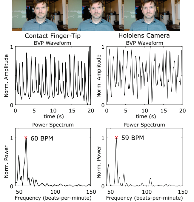
Figure 5: Examples of pulse waveforms from the finger-tip sensor and iPPG measurements. Top) The PPG waveforms. Bottom) The power spectra of the BVP signal and the detected HR. Thumbnail example frames from the Hololens video capture are shown above.
