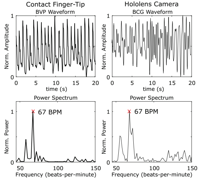
Figure 6: Examples of pulse waveforms from the finger-tip sensor and iBCG measurements. Top) The BCG waveform from the Hololens and the PPG waveform from the finger-tip sensor. Bottom) The power spectra of the signals and the detected HR.
