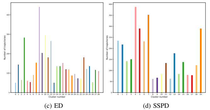
Figure 11. ED versus SSPD clustering results
