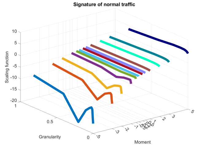
Fig. 10. Scaling function for regular traffic
