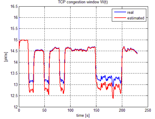
Fig. 15. TCP congestion window W(t) - CFC attack
