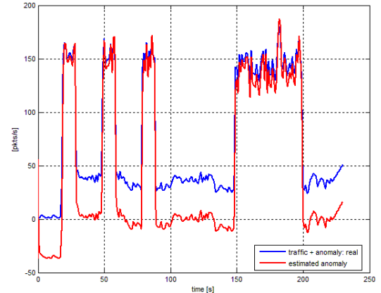
Fig. 17. Estimation with real traffic replay - CFC attack
