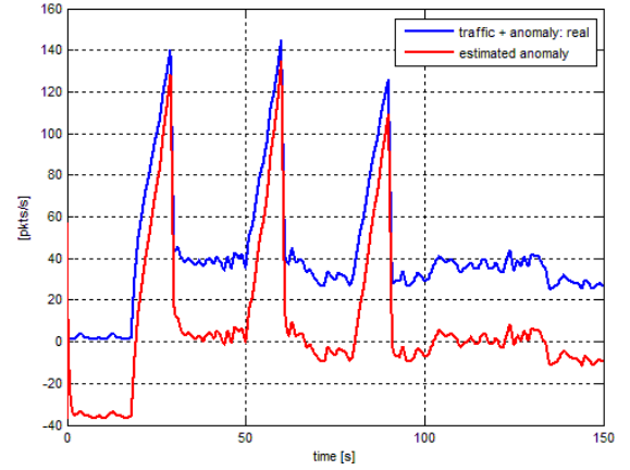
Fig. 20. Estimation with real traffic replay - PFC attack
