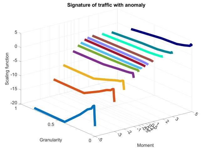
Fig. 11. Scaling function for traffic with PFC anomaly
