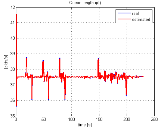
Fig. 16. Queue length q(t) - CFC attack
