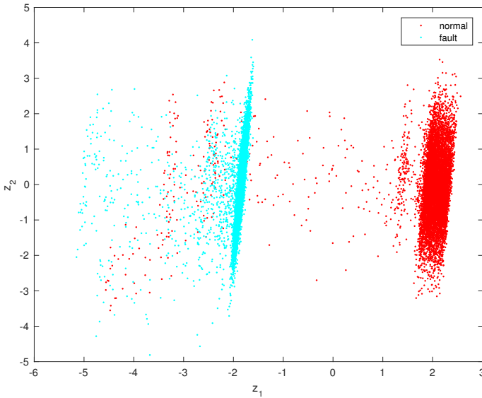
Figure 8: Reduced feature space z_1 vs z_2
