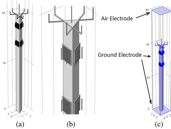
Figure 3: Model for the electrostatic simulation: (a) complete pylon; (b) antennas; (c) computation volume and electrodes.
