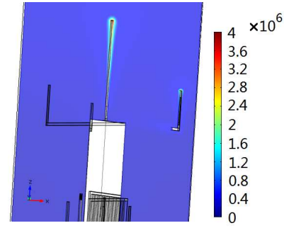
Figure 4: Electrostatic field near the top of the pylon (V/m).
