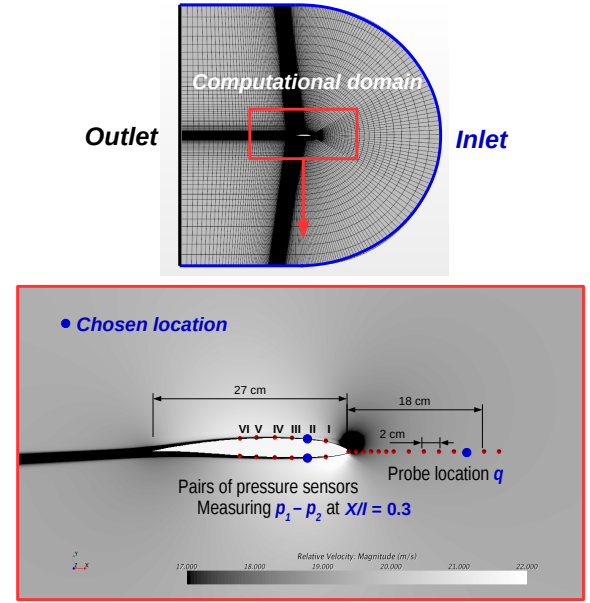
Figure 3: CFD computational domain of SD2048 Airfoil with port pair measuring pressure difference and pitot tube measuring dynamic pressure.
