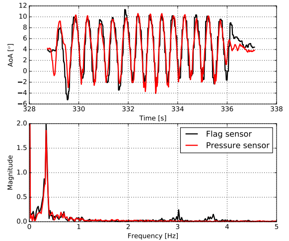
Figure 10: High frequency oscillations in flight test provoked by command input in calm atmosphere
