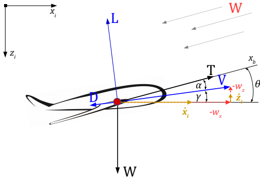
Figure 8: Longitudinal equations of motion.
