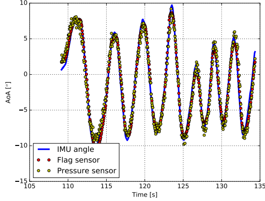
Figure 7: Results of calibration from wind tunnel experiment
