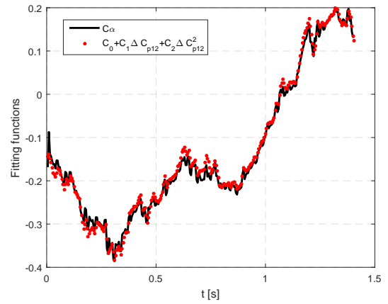
Figure 4: Curve fitting for numerical simulations ( Re = 340,000 ).
