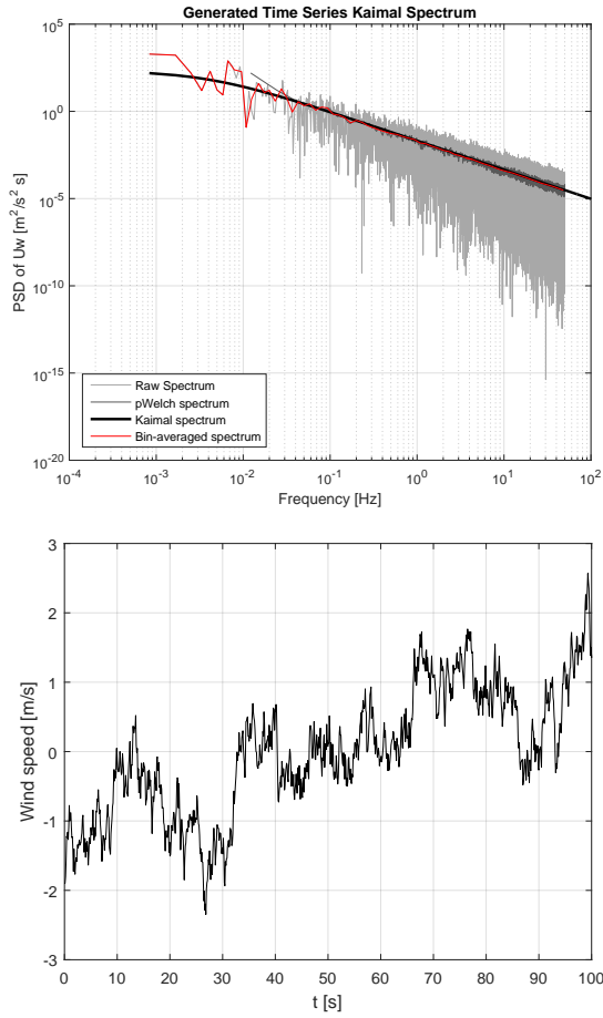
Figure 2: Generated time series of Kaimal spectrum as an input for URANS simulations.
