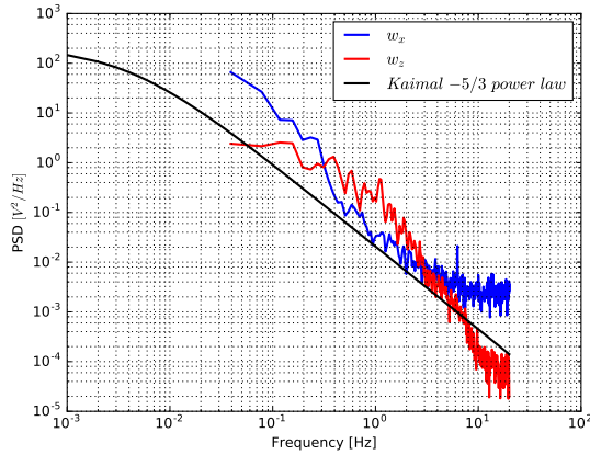
Figure 14: Estimated wind spectrum
