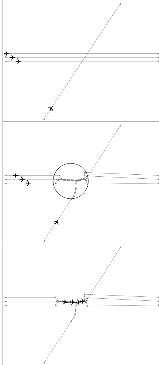
Figure 20: Results of the third algorithm. Top: initial scenario, central trajectories are 100 NM long, and spaced by 5 NM. Center: aggregated flight plans, area to regulate represented by the circle. Bottom: aircraft following new flight plans.
