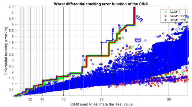
Figure 8. Galileo E1C, comparison of SQMs based on simple ratio metrics for different monitors distributions.
