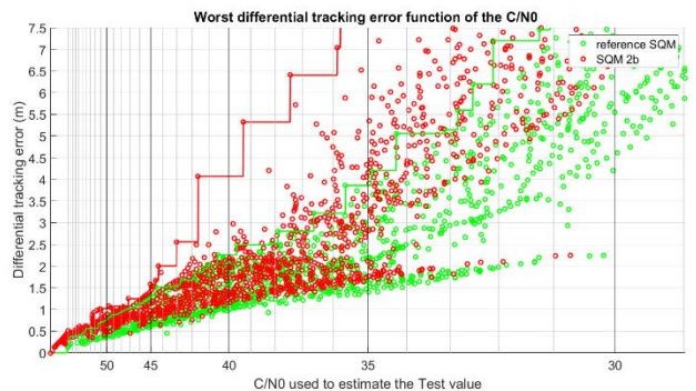
Figure 4. Comparison of two SQMs performance.
