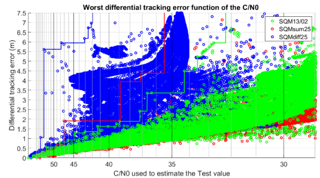
Figure 9. Galileo E1C, comparison of SQMs based on simple, difference and sum ratio.
