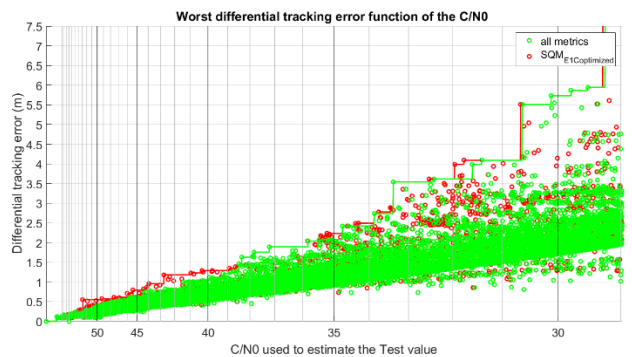
Figure 13. Optimized SQM and 100 metrics SQM comparison. Galileo EIC.
