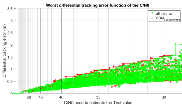
Figure 14. Optimized SQM and 40 metrics SQM comparison. Galileo E5a.
