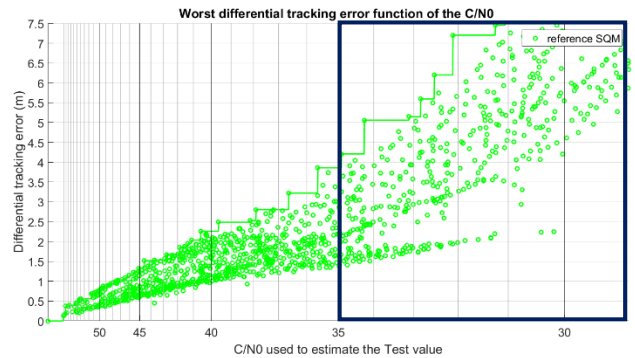
Figure 3. Example of worst differential tracking error function of the equivalent C/N_0 .
