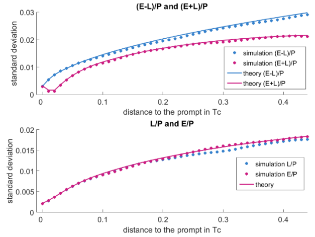
Figure 1. Theoretical and simulated metric standard deviations on a BPSK(1) autocorrelation function.
