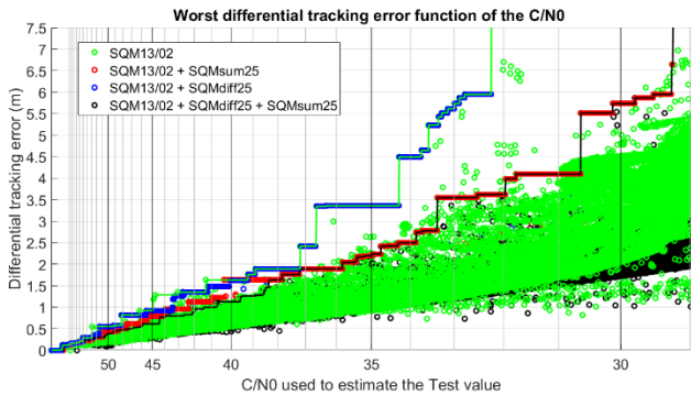
Figure 11. Galileo EIC combination of simple, difference and sum ratio SQMs comparison.
