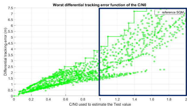
Figure 2. Example of worst differential tracking error function of Test_{MDE} .
