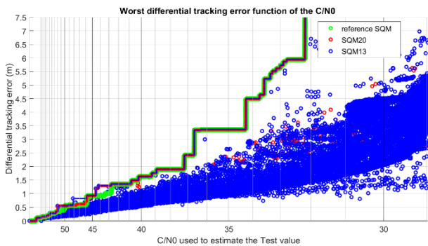
Figure 7. Galileo E1C simple ratio SQMs comparison on different areas.
