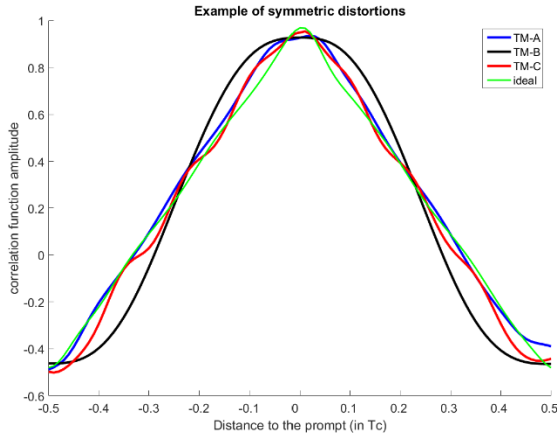
Figure 10. Example of symmetric distortions on Galileo EIC difficult to detect with difference ratio metrics.
