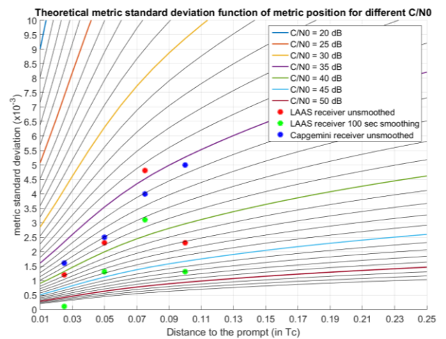
Figure 5. Example of reference station metric standard deviations compared to theoretical values.
