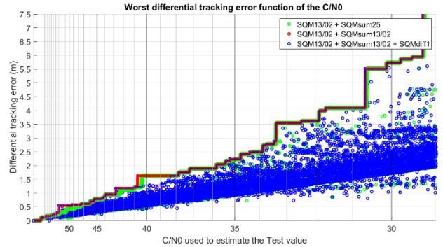
Figure 12. Different simple ratio metrics used with sum ratio metrics. Galileo EIC.
