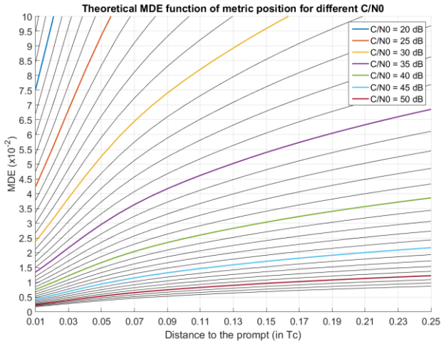
Figure 6. Simple ratio metric performance thresholds for different C/N_0 and different distance to the prompt.
