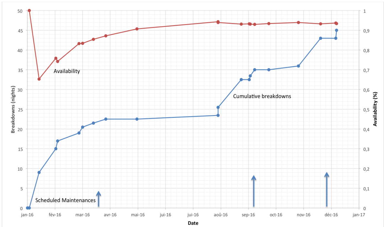
Figure 7: System efficiency statistics of TCA and TCH (see text): the overall efficiency increased to more than 90% after repair in January 2016. The various breakdown (instrumental, hardware or software), are shown together with their duration. The scheduled maintenance periods (March and September for TCA, November for TCH) are also shown with their duration (arrows), but are not taken into account for the computation of the system efficiency. Weather interruptions have not been taken into account.
