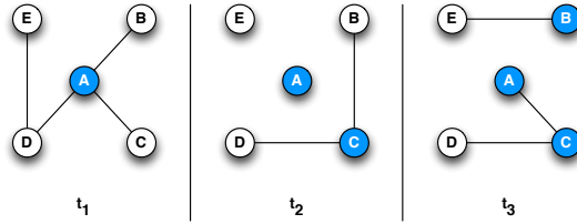
Figure 3: Dynamics of temporal random walks
