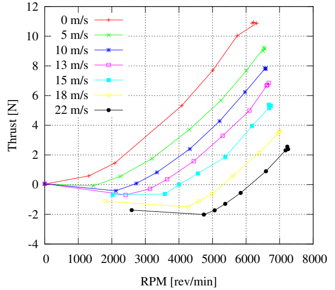
Fig. 4: Thrust versus RPM at different airspeed from wind tunnel experiment.
