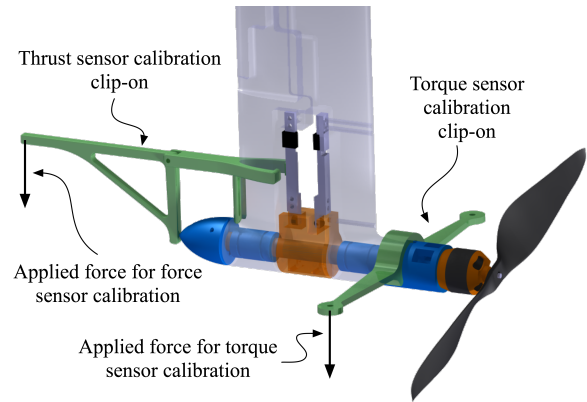
Fig. 7: Clip-on calibration parts.
