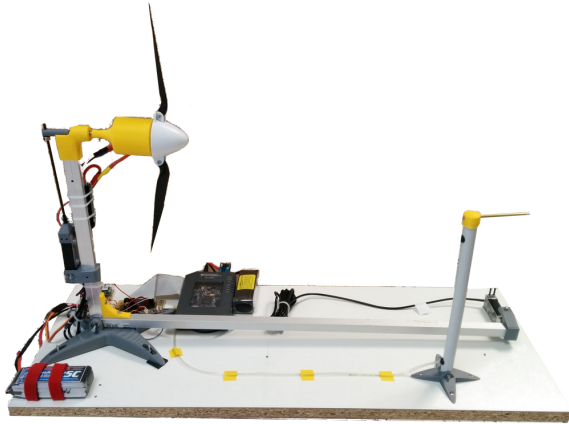
Fig. 3: First test bench version.
