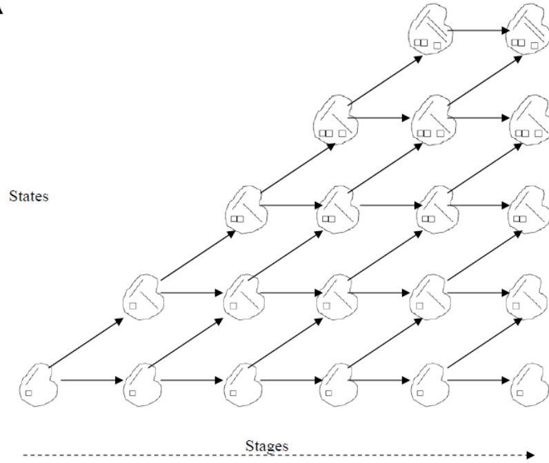
Figure 1: Dynamic Programming Decision Graph
