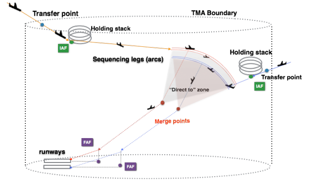
Fig. 2: ML-PM system for parallel runways operation
