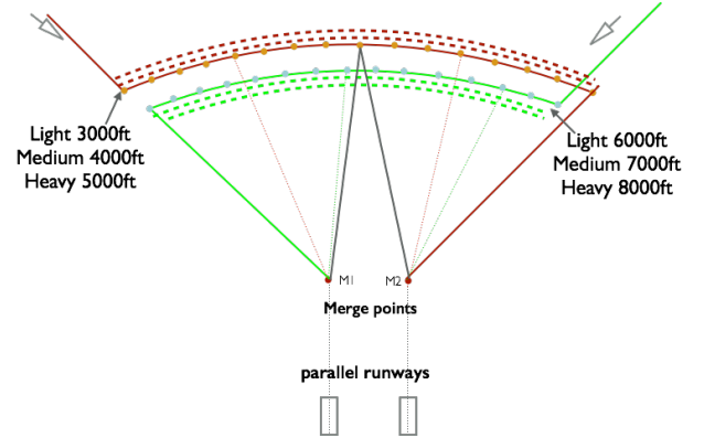
Fig. 3: Horizontal plan of ML-PM system
