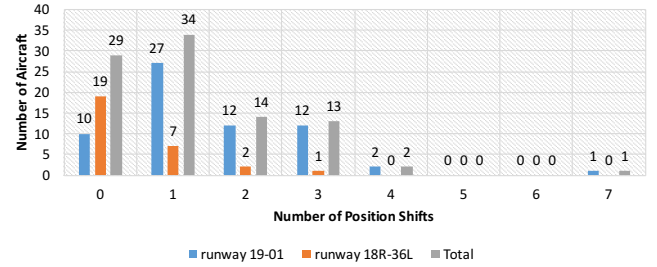
Figure 9. Position shift performance in ML-PM scenario
