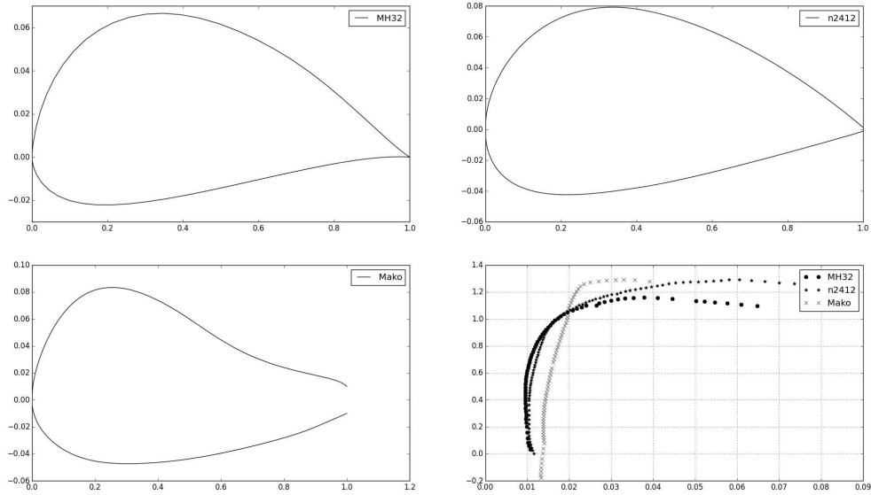
Fig 3: Candidate airfoils
