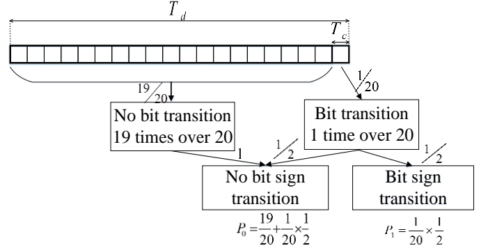
Fig. 7: Scheme to determine the probability of detection (GPS L1 C/A)
