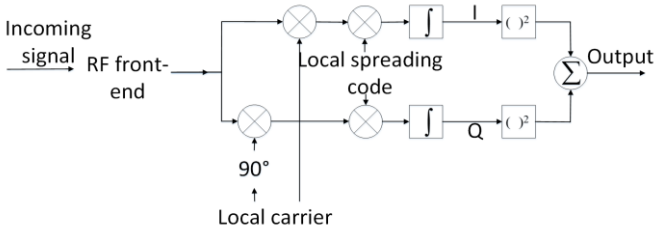
Fig. 1: Block diagram of the serial search acquisition
