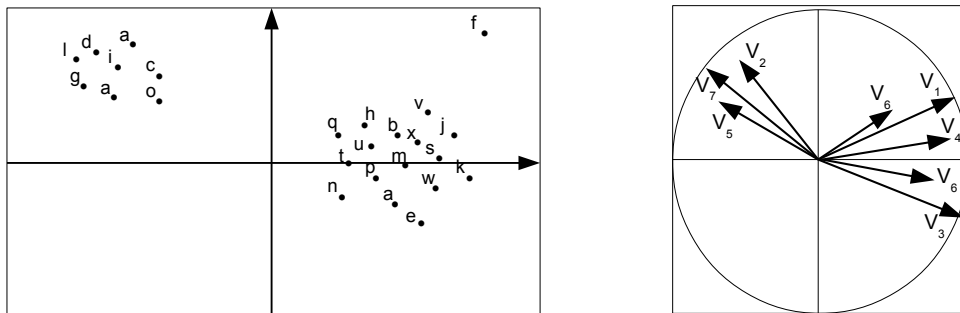
Figure 2: Representation of individuals (left panel) and variables (right panel) onto a plane defined by two principal component factors.
