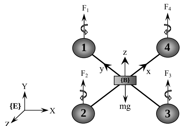
Fig. 1. Quadrotor scheme
