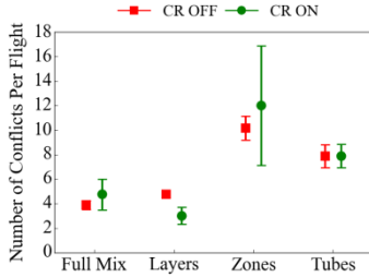
b) Effect of Conflict Resolution (CR)
