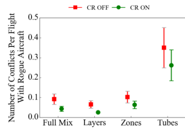
Figure 14: Number of conflicts per flight with rogue aircraft
