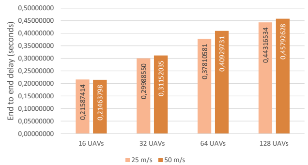
Fig. 13: Analysis of end to end delay on IEEE 802.15.4 with Star configuration.
