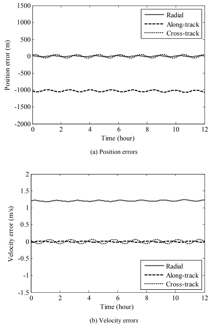
Fig. 5. Evolution of the radial, along-track, and cross-track position and velocity errors of the adaptive HLS filter.
