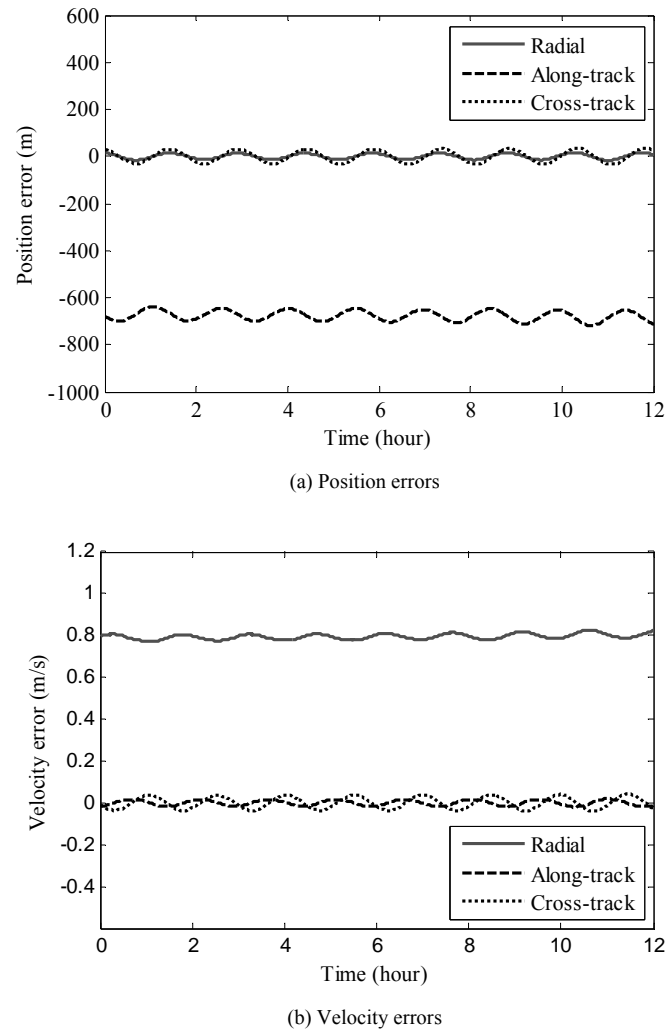
Fig. 7. Evolution of the radial, along-track, and cross-track position and velocity errors after the drift estimation.
