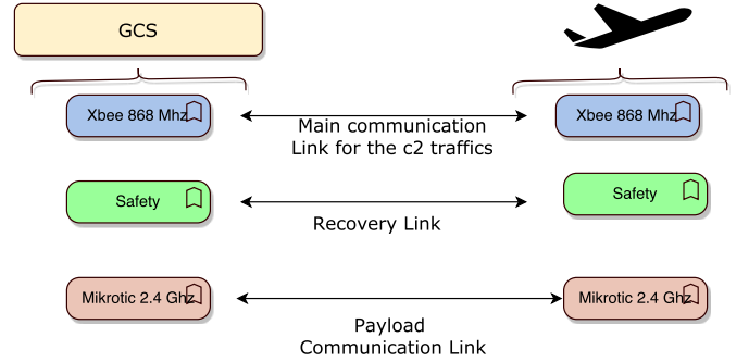
Figure 7. Communication Links Between Nodes
