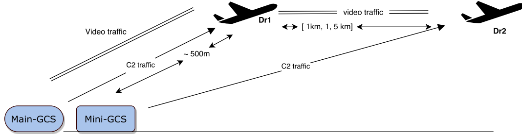
Figure 8. UAANET Real World Experiment Scenario
