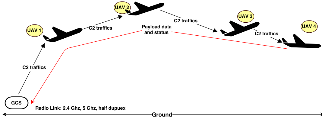
Figure 1. UAANET Architecture
