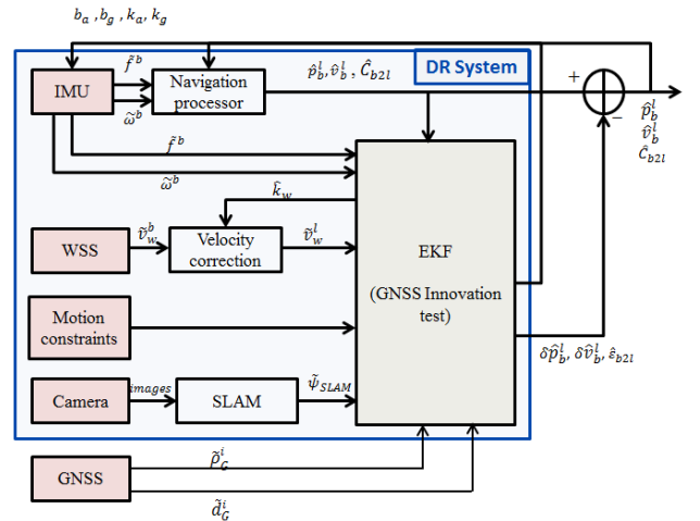
Figure 2: Filter architecture
