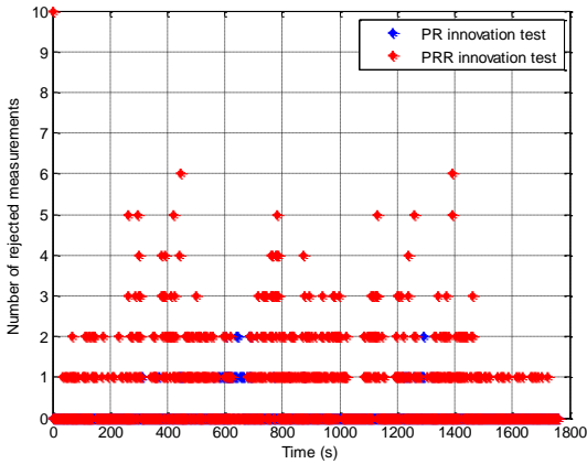
Figure 6: Number of removed SVs with innovation test
