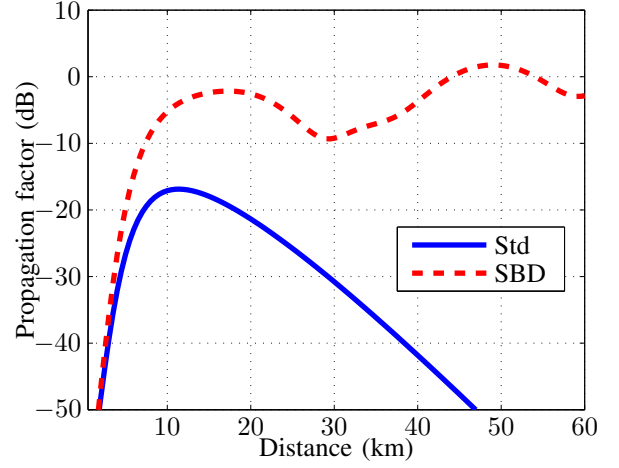
Fig. 4. Propagation factors with respect to distance just above the sea level corresponding to the standard atmosphere (Std) and to a surface-based duct (SBD).
