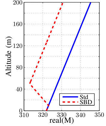
Fig. 2. The modified refractivity of the two samples corresponding to the standard atmosphere (Std) and to a surface-based duct (SBD).
