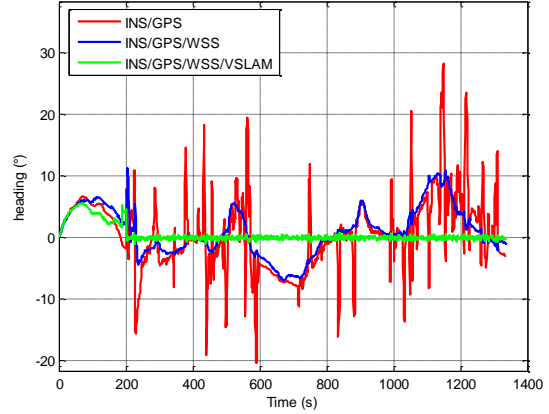
Figure 8: Heading error
