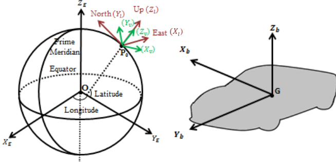
Figure 2: Reference frames
