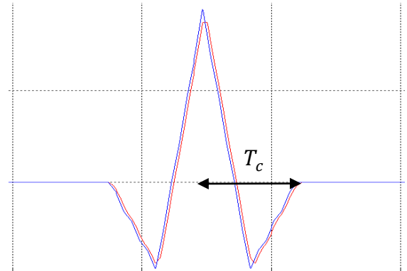
Figure 19. Impact of the digital distortion 5 on the signal (top), and on the correlation function (bottom).
