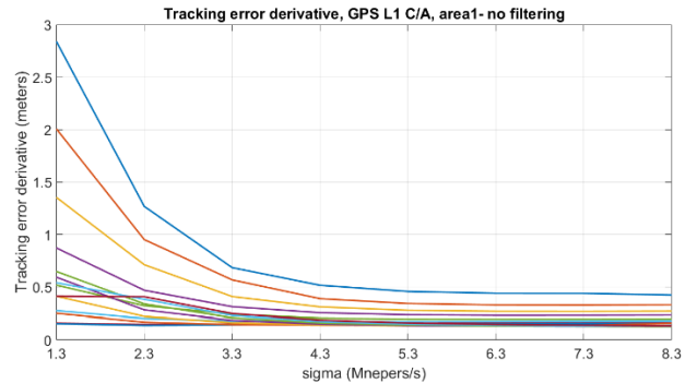
Figure 7. \Delta_{err\_dist} associated to the Threat Space grid from Figure 6. (GPS L1 C/A ICAO TM)
