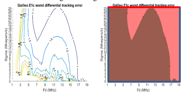
Figure 2. Worst differential tracking error for different signal distortion parameters. On the right, only the 1m limit is shown. Blue limits give the remaining conservative TM. Red limit underline that the TM cannot be bound for high sigma values. Galileo E1C
