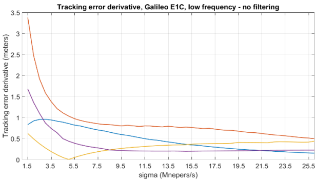
Figure 9. \Delta_{err\_dist} associated to zone1 Threat Space grid from Figure 8. (Galileo E1C, area1 of the proposed TM)
