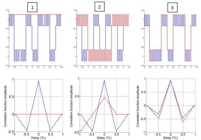
Figure 22. CBOC signal affected by different digital distortions on the top and associated correlation function on the bottom.
