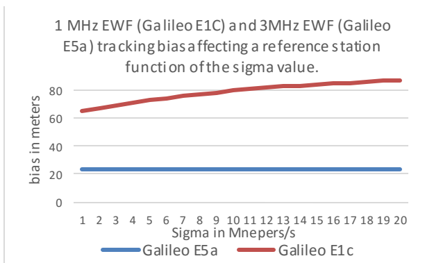
Figure 1. 1MHz (Galileo E1C) and 3MHz (Galileo E5a) EWF consequences on a standalone receiver without applying filtering
