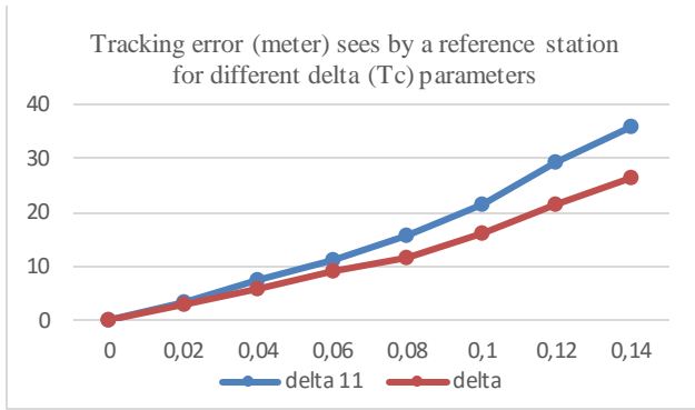
Figure 23. Tracking error for TM-A1 and TM-A2 and different delta values ( \Delta and \Delta_{11} ).
