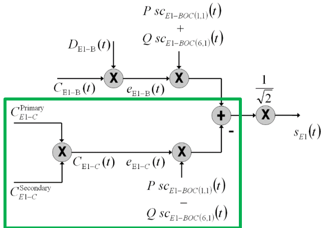
Figure 18. Galileo E1 signal generation block scheme [8]
