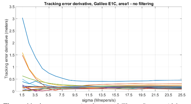
Figure 11. \Delta_{err\_dist} associated to zone3 Threat Space grid from Figure 8. (Galileo E1C, area1 of the proposed TM)
