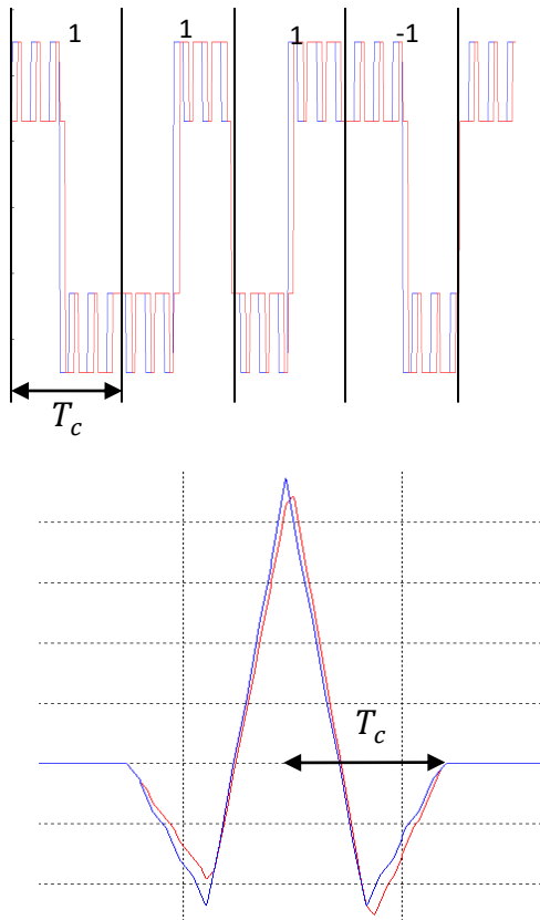
Figure 20. Impact of the digital distortion 4 on the signal (top), and on the correlation function (bottom).
