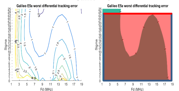
Figure 3. Worst differential tracking error for different signal distortion parameters. On the right, only the 1m limit is shown. Blue limits give the remaining conservative TM. Red limit underline that the TM cannot be bound for high sigma values. Galileo E5a
