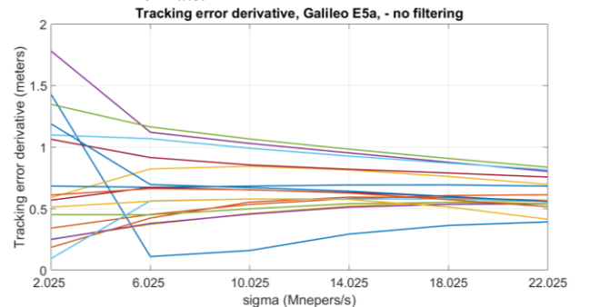
Figure 13. \Delta_{err\_dist} associated to the Threat Space grid from Figure 12. (Galileo E5a, area1 of the proposed TM)
