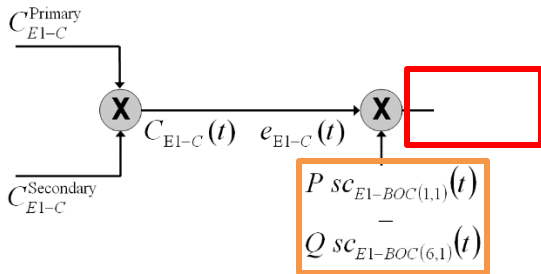
Figure 21. Galileo E1C signal generation and digital distortions
