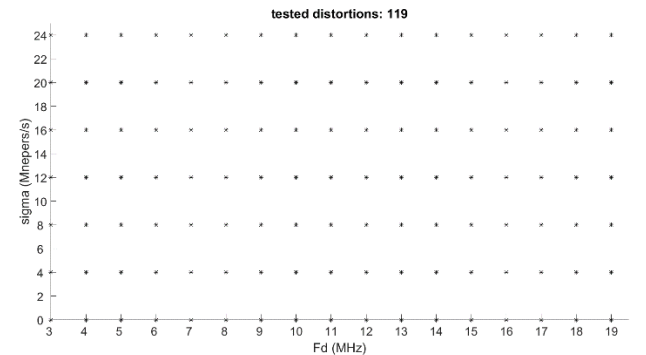
Figure 12. Example of a Threat Space grid. (Galileo E5a, area1 of the proposed TM)
