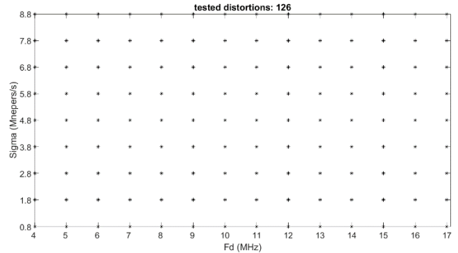
Figure 6. Example of a Threat Space grid. (GPS L1 C/A ICAO TM)
