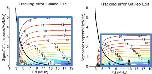
Figure 4. Tracking error affecting the reference in meter generated by a 2 nd order filtering function of \frac{\sigma}{(f_d)^2} and f_d . Blue rectangles represent area2 limits, black lines area1 upper limits.
