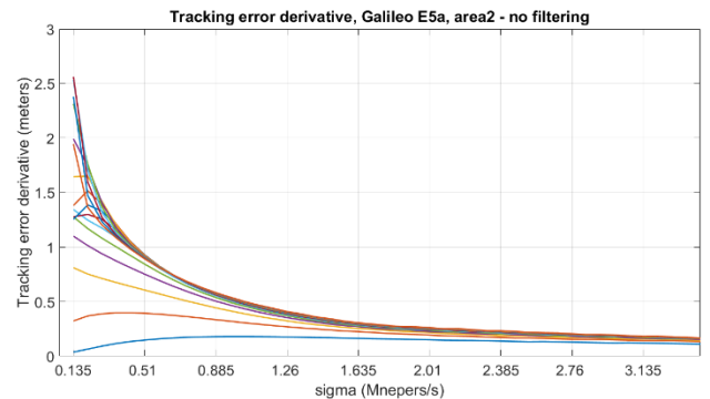
Figure 16. \Delta_{err\_dist} values (Galileo E5a, area2 of the proposed TM)
