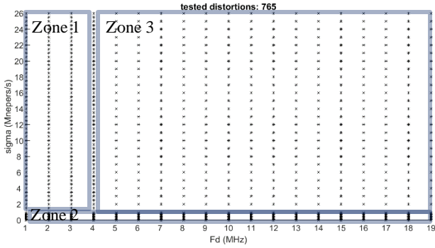
Figure 8. Example of a Threat Space grid. (Galileo E1C, area1 of the proposed TM)
