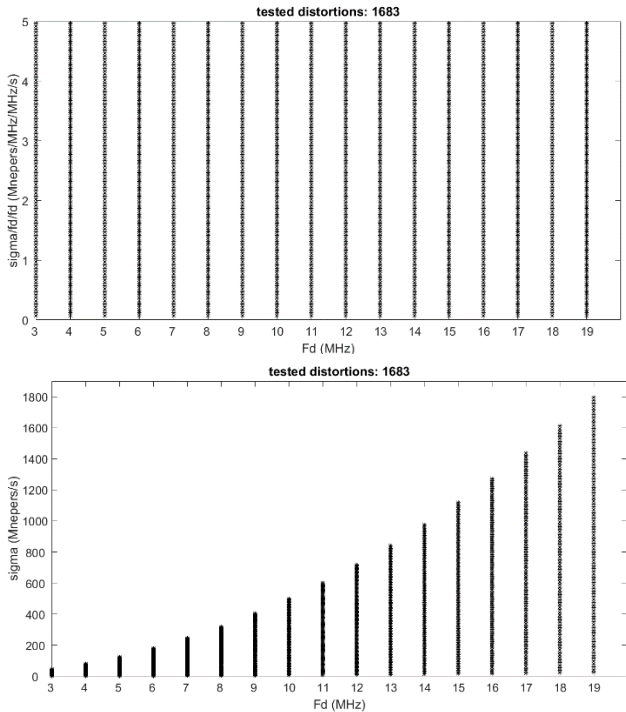
Figure 14. Example of a Threat Space grid. (Galileo E1C, area2 of the proposed TM). On the top in the \frac{\sigma}{f_d^2} representation, on the bottom in the \sigma representation.
