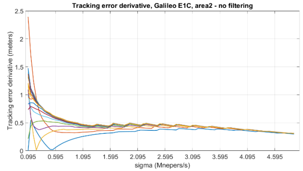
Figure 15. \Delta_{err\_dist} associated to the Threat Space grid from Figure 10. (Galileo E1C, area2 of the proposed TM)
