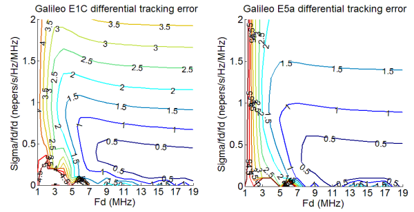
Figure 5. Differential tracking error in meter generated by a second order filtering function of \frac{\sigma}{(f_d)^2} and f_d
