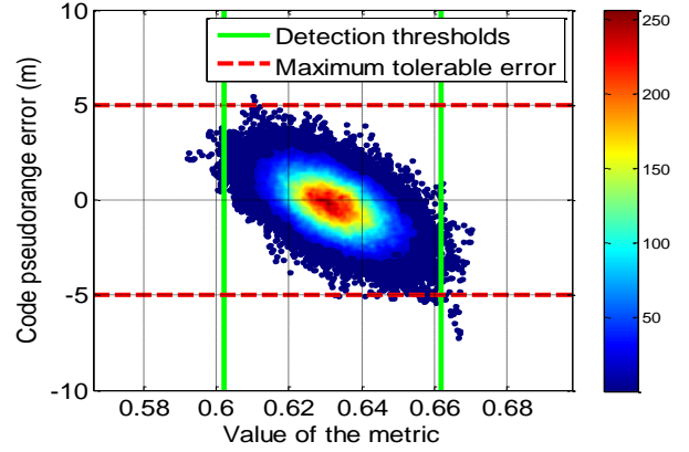
Figure 11 Correlation between code pseudorange error and non coherent simple ratio metric ( M_3 )
