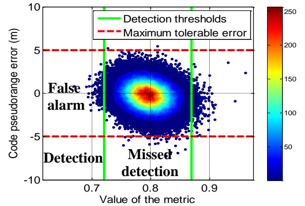
Figure 5 Correlation between code pseudorange error and value of the raw simple ratio metric ( M_1 ) for BPSK
