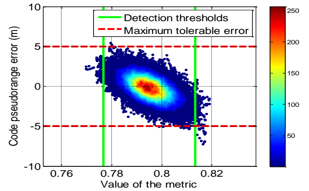
Figure 6 Correlation between code pseudorange error and value of the simple ratio metric ( M_1 ) after smoothing the correlator outputs for BPSK
