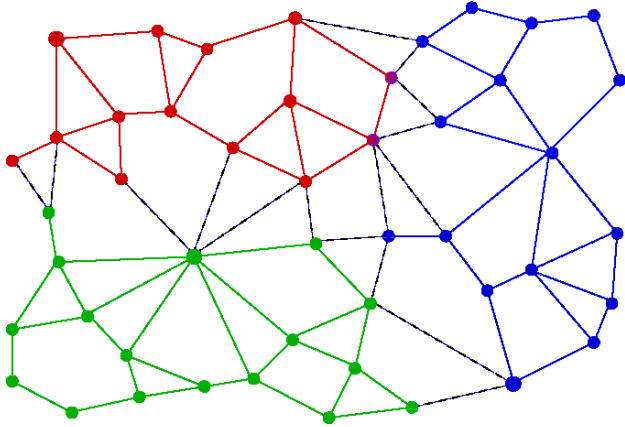
Figure 10. Example of a partition of a graph into three connected components
