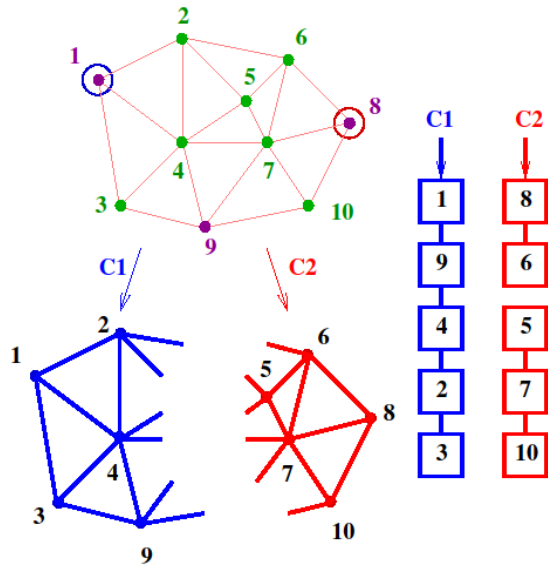
Figure 12. Example of the coding graph partitioning for one time period
