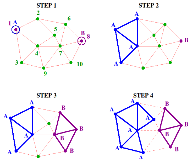
Figure 13. Greedy heuristic is used to create initial partitions
