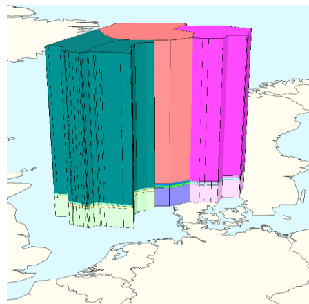
Figure 17. DAC level-2: 6 sectors and 6 SBBs
