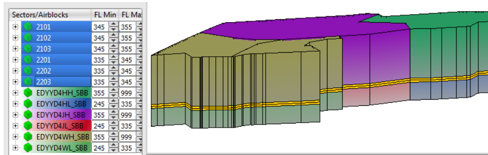
Figure 18. DAC level-2 scenario airspace components vertical limits
