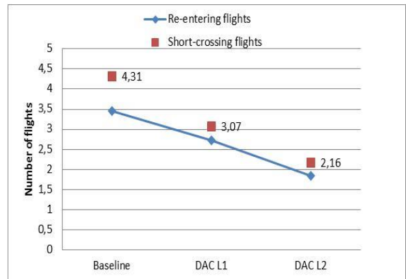
Figure 22. Re-entering and short-crossing flights
