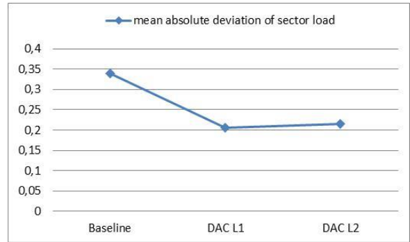
Figure 21. Sector load balancing criteria
