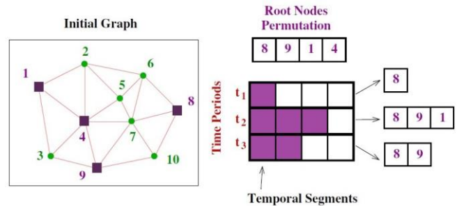
Figure 11. Chromosome structure
