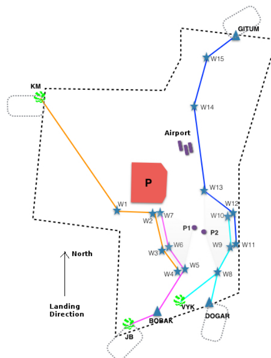
Figure 4 Beijing Arrival Chart with M-PM System
