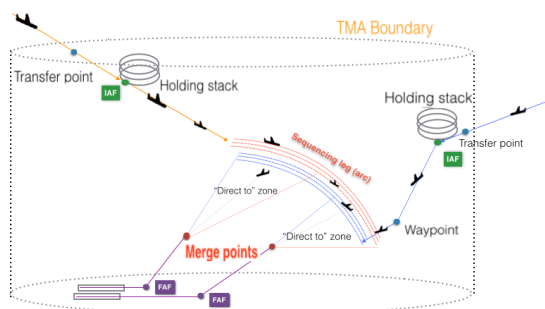
Figure 2 Advanced PM System for Parallel Runways
