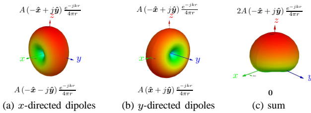
Fig. 1. Hemispherical radiation pattern: contribution of x -directed and in-quadrature y -directed dipoles in the electric field.
