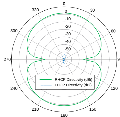
Fig. 5. Directivity pattern (dBi) of one mode in the xOz plane at 0.59 GHz.
