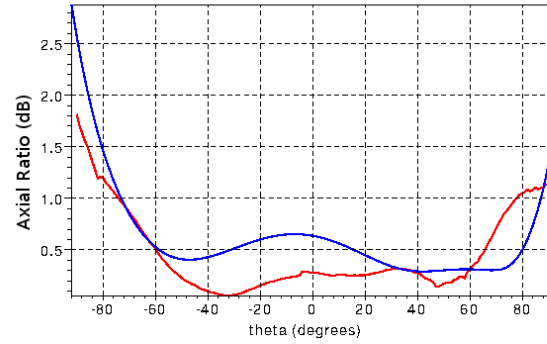
Fig. 14. Axial ratio (dB) in the xOz plane for \alpha_f = -j : measurement (red), simulation (blue).
