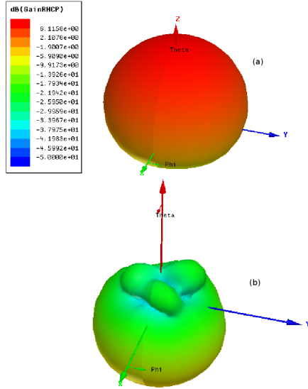
Fig. 11. 3D gain pattern (dBi) for \alpha_f = -j : (a) RHCP, (b) LHCP.
