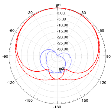
Fig. 17. Directivity pattern (dBi) for RHCP (red) and LHCP (blue) polarizations, in the xOz (solid line) and yOz (dashed line) planes.
