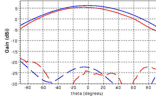
Fig. 13. Gain Pattern (dBi) in the xOz plane for \alpha_f = -j : RHCP measurement (red line), RHCP simulation (blue line), LHCP measurement (dashed red line), LHCP simulation (dashed blue line).
