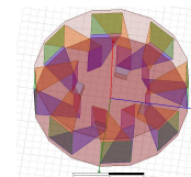
Fig. 15. Symmetrical antenna structure with eight turns.
