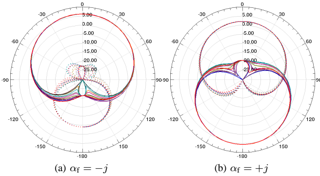
Fig. 12. Gain pattern (dBi) for azimuth angles \phi = \{0, 15^\circ, \dots, 180^\circ\} .
