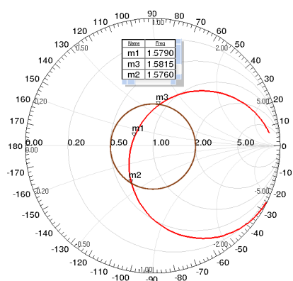
Fig. 16. Reflection coefficient S_{11} on Port 1 of the antenna for a reference impedance of 50 \Omega . The brown circle indicates the area where VSWR \leq 2 .
