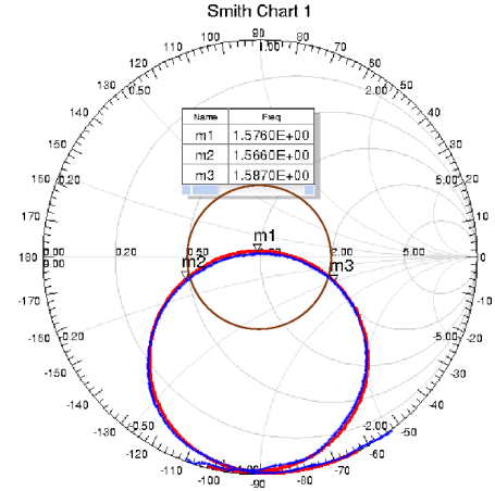
Fig. 10. Reflection coefficient S_{11} on Port 1 of the antenna for a reference impedance of 50 \Omega : measured (blue), simulated (red). The brown circle indicates the area where VSWR \leq 2 .
