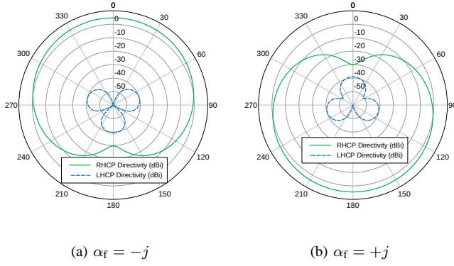
Fig. 6. directivity pattern (dBi) of both modes in the xOz plane at 0.59 GHz.
