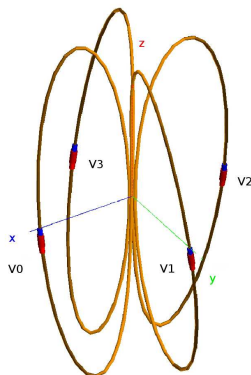
Fig. 4. Four-turns helical ring antenna.
