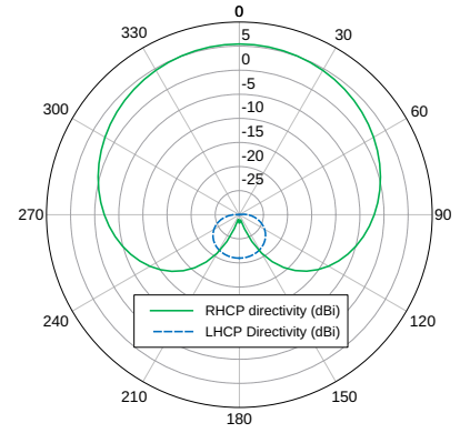
(b) Directivity pattern (dBi) in the xOz plane for \alpha_f = -j at 0.59 GHz.
