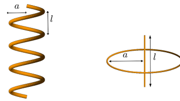
(a) helix (b) equivalent model for one turn
