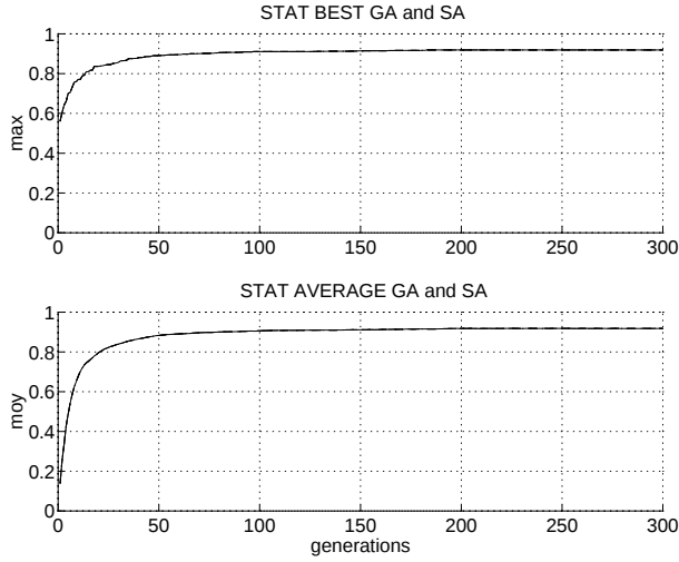
Figure 20: Fitness evolution
