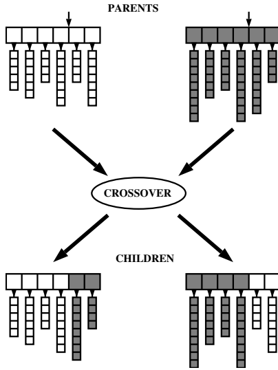
Figure 17: Crossover operator
