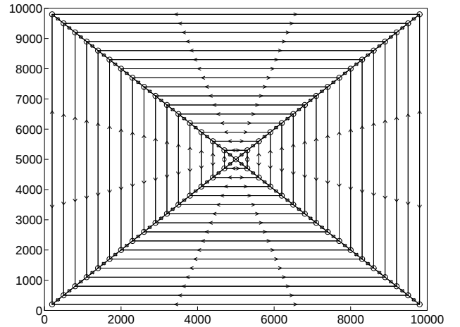
Figure 19: Test network
