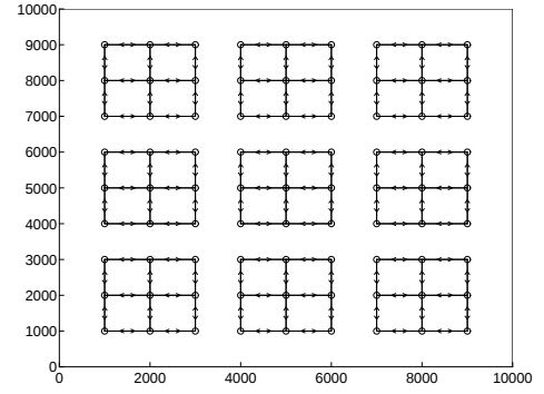
Figure 14: Square network
