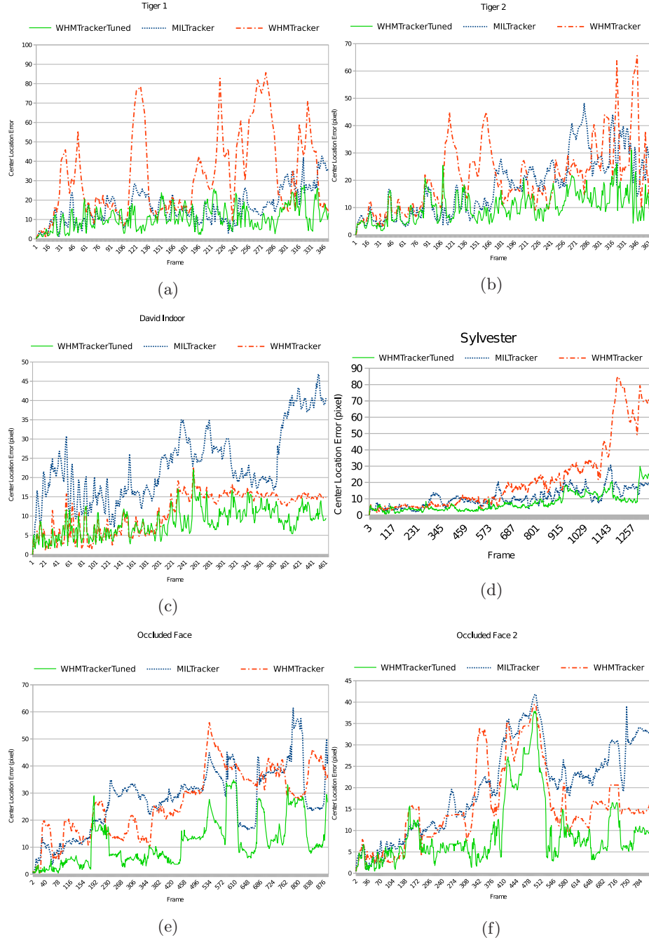
Fig. 3: Figures 3a , 3b, 3c, 3d, 3e and 3f show a comparison among the tracker in [3], WHMTracker and Tuned WHMTracker for Tiger1 , Tiger2 , DavidIndoor , Sylvester , OccludedFace and OccludedFace2 video clips, respectively.
