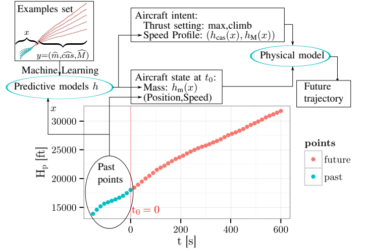
Figure 5: This figure describes how the future trajectory is predicted by applying Machine Learning techniques. The examples set is used to build predictive models ( h_m , h_{cas} , h_M ). When a fresh trajectory is observed, the input variables x are computed from the observed points and the predictive models are used to predict the mass and the speed profile.
