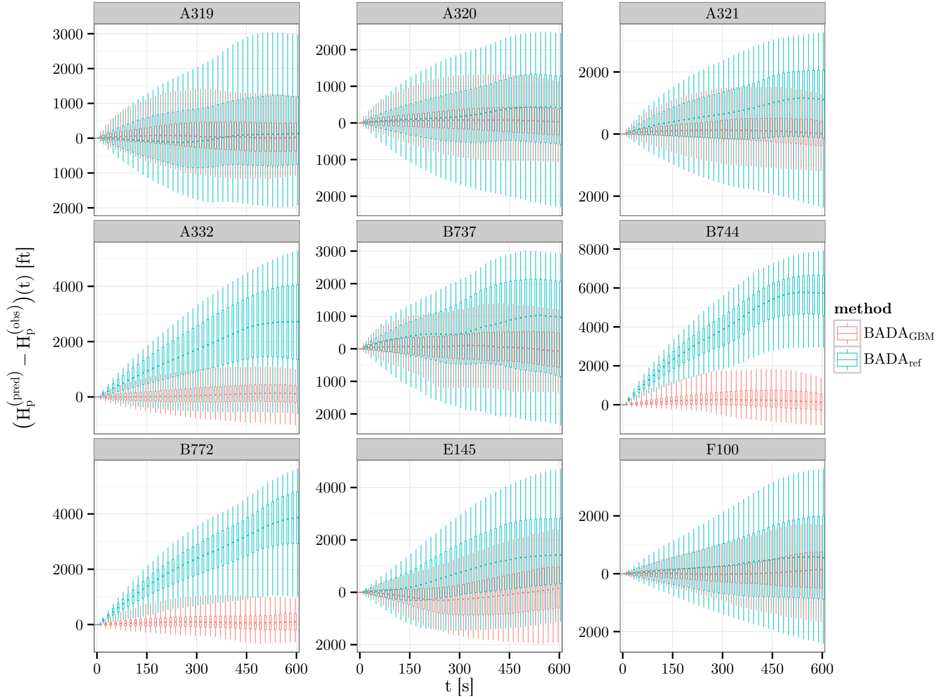
Figure 6: This figure portrays the error on the altitude obtained by BADA_{\text{ref}} and BADA_{\text{GBM}} for nine different aircraft types. Each time step, a boxplot shows the 5 %, 25 %, 50 %, 75 % and 95 % quantiles. The whiskers (resp. box) of the boxplot contains 90 % (resp. 50 %) of the data.
