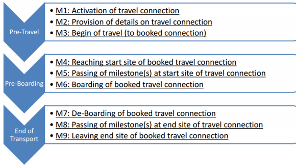
Fig. 5: MetaCDM Milestones.
