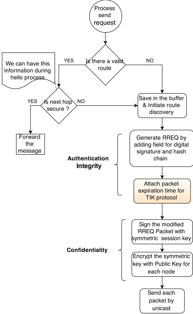
Figure 11. Flow chart for process send request
