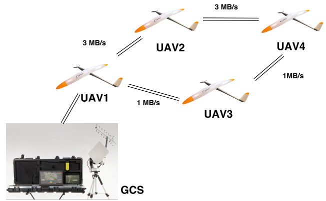
Figure 13. Use case where hop count metric is not sufficient
