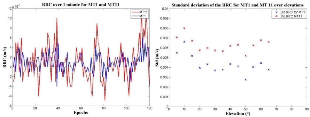
Fig. 8 – RRC over 1minute (left) and Standard deviation of RRC (right) for MT1 (blue) and MT11 (red)
