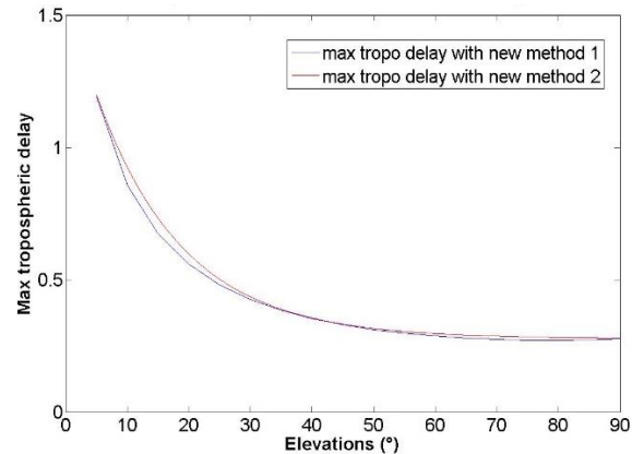
Figure 10 - \mu_{max} with the 2 new methodologies
