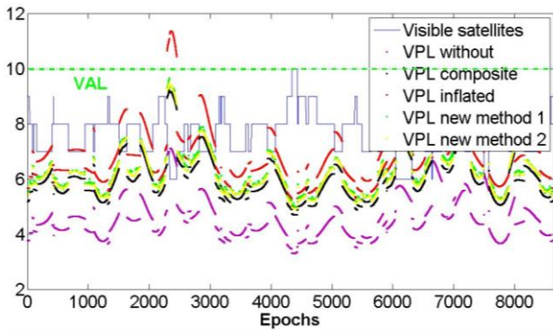
Figure 11- VPLs with D_{TH}=5km for GPS constellation only
