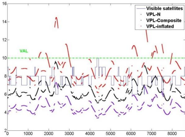
Figure 6 - VPLs with D_{TH}=10\text{km} for GPS constellation only
