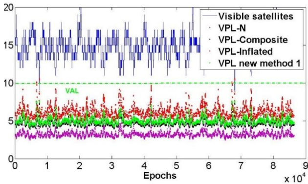
Figure 9-VPLs with D_{TH}=5\text{km} for GPS + GAL constellations
