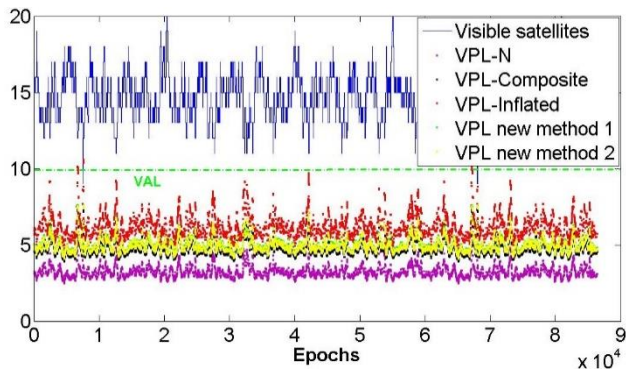
Figure 12 -VPLs with D_{TH}=5km for GPS + GAL constellations
