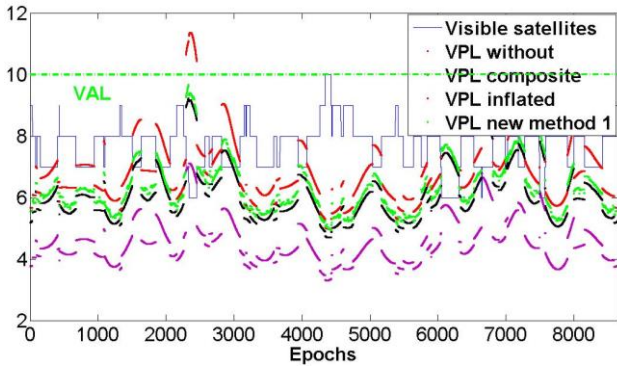
Figure 8 - VPLs with D_{TH}=5\text{km} for GPS constellation only
