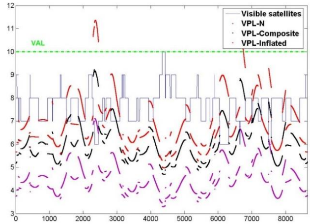
Figure 4 - VPLs with D_{TH}=5\text{km} for GPS constellation only
