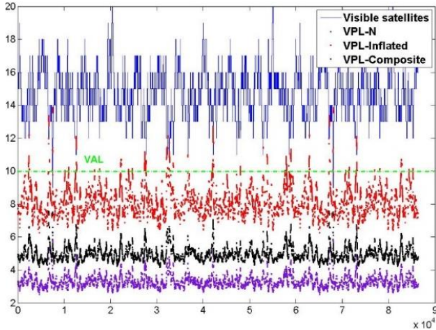
Figure 7 - VPLs with D_{TH}=10\text{km} for GPS + GAL constellations
