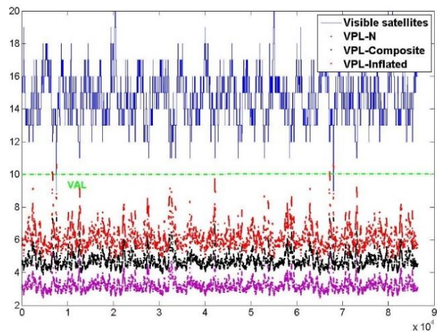
Figure 5- VPLs with D_{TH}=5\text{km} for GPS + GAL constellations
